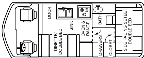
FLOOR PLAN 23'-3
