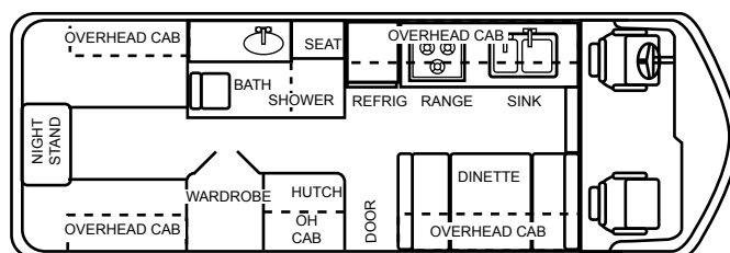
SIDE BATH
