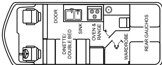
FLOOR PLAN 23'-5
