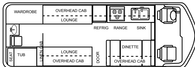
REAR BATH
