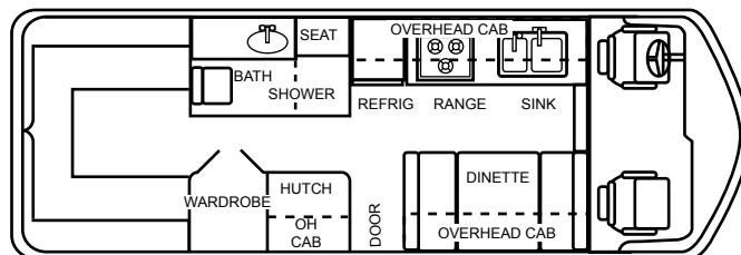
REAR DINETTE
