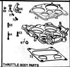
THROTTLE-BODY PARTS
