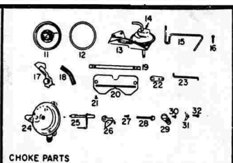
CHOKE PARTS
